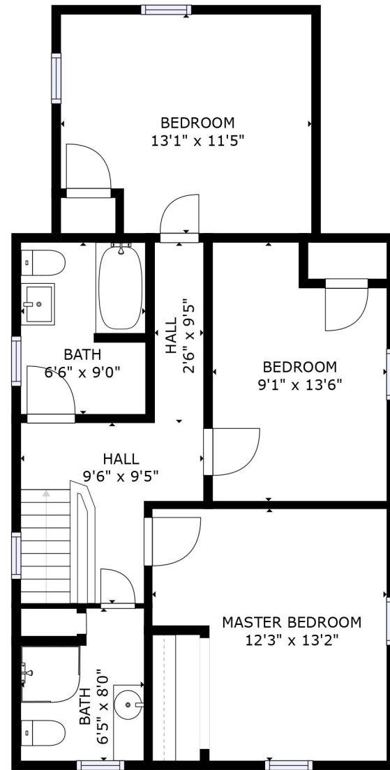
FLOOR 2
